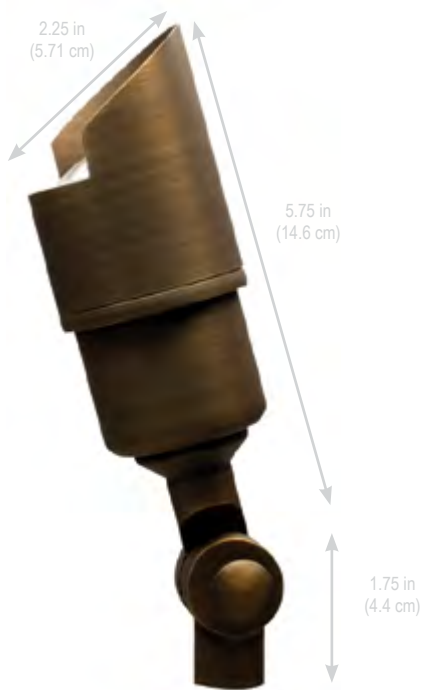
BL110-LED6W (6 watt MR16 LED lamp included)
