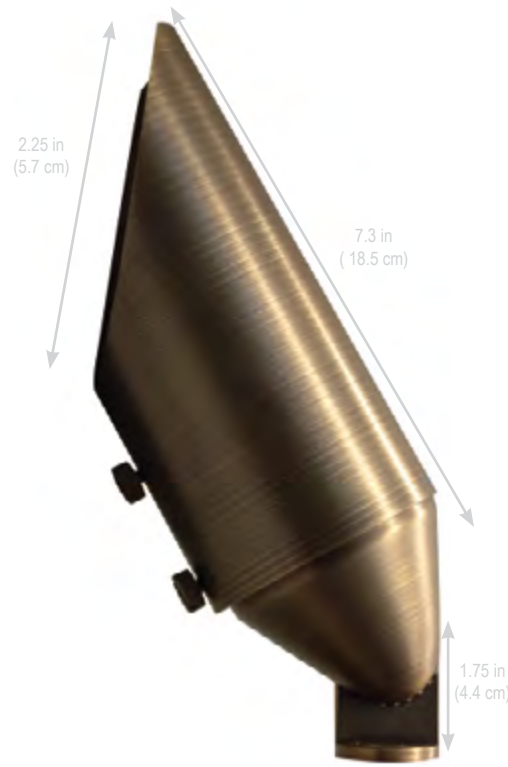
BL900-LED6W (6 watt MR16 LED Lamp included)
